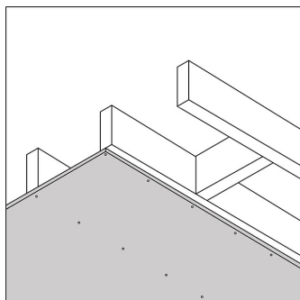
Plasterboard
